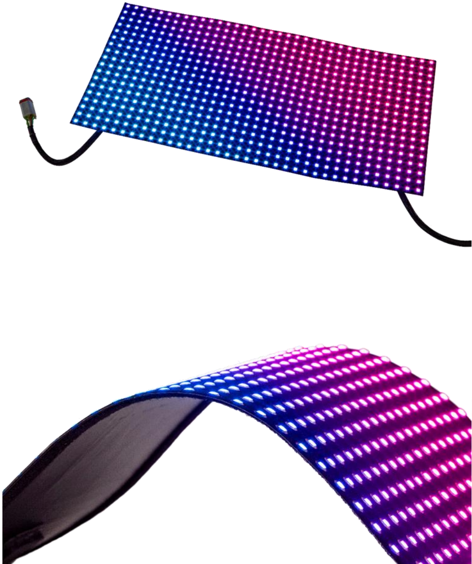
Figure 1: ledTec.flex banner P16 4000
